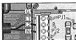
2 phase connection
