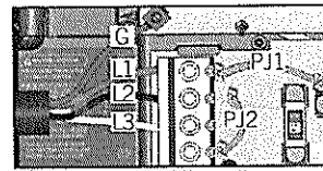
3 phase Delta connection
